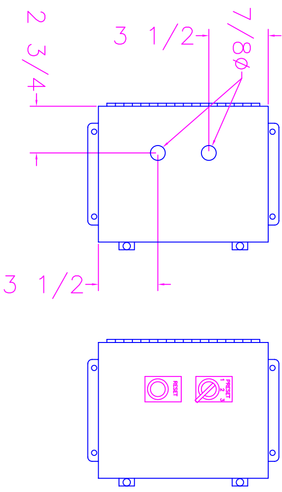
ENCLOSURE MODIFICATION & OPERATOR LAYOUT
